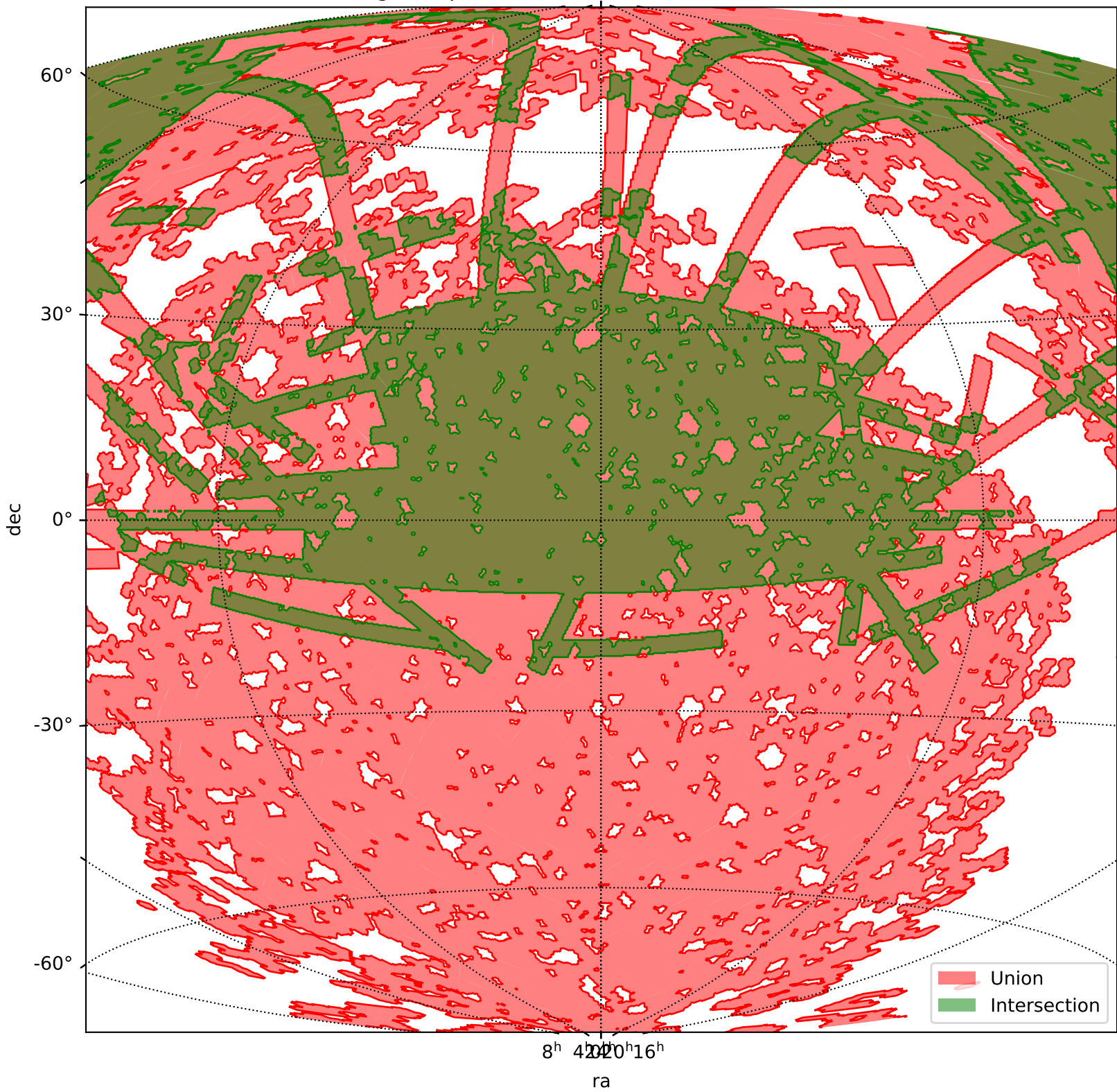
Logical operations between SDSS and GALEX
